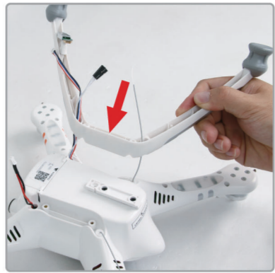
1.2 Install the right skid, carefully pull the cables and the antenna through the holes in the landing gear.
